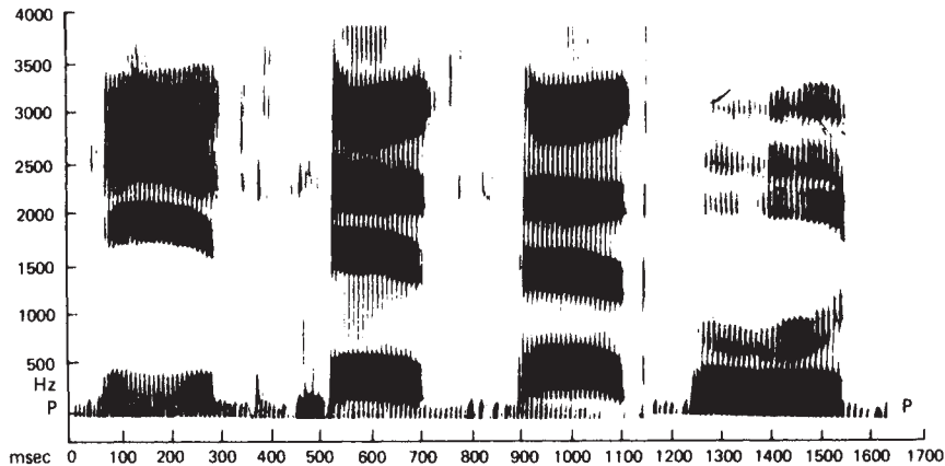
FIGURE 8.2 | A spectrogram of the words heed , head , had , and who'd , spoken with a British accent (speaker: Peter Ladefoged, February 16, 1973).
