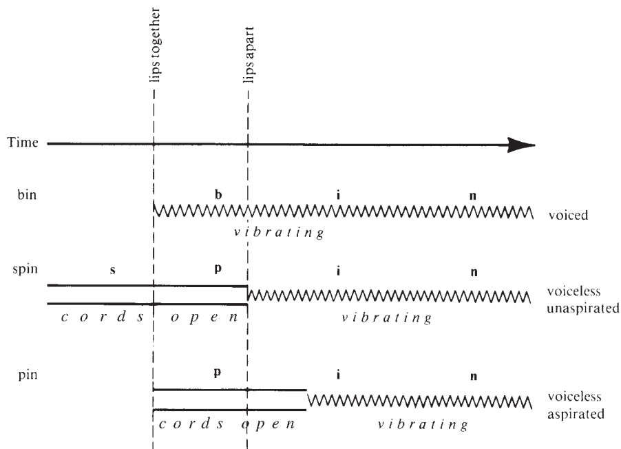
FIGURE 4.2 | Timing of lip closure and vocal-cord vibrations for voiced, voiceless unaspirated, and voiceless aspirated bilabial stops [b], [p], [p h ].
