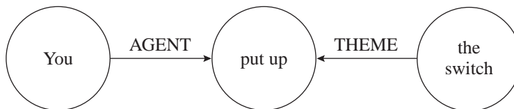
FIGURE 8.6 | Semantic network for You put up the switch .
